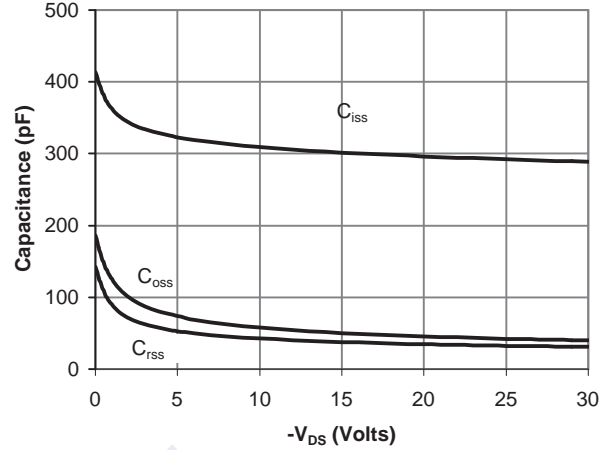
Figure 8: Capacitance Characteristics 370
