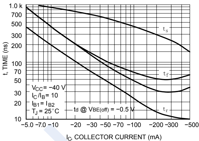
Figure 4. Switching Time
